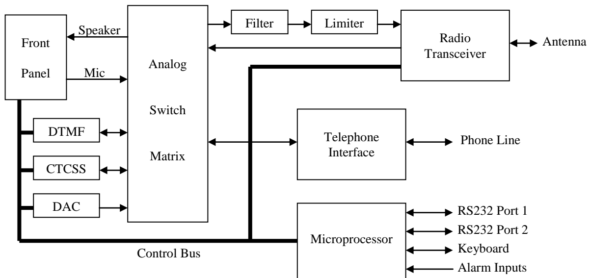
PEOPLE FINDER II Base Block Diagram
